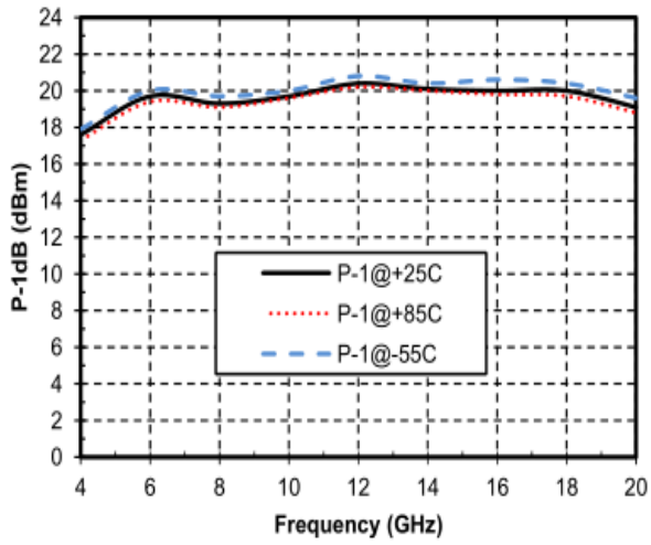
P-1dB vs. Frequency
