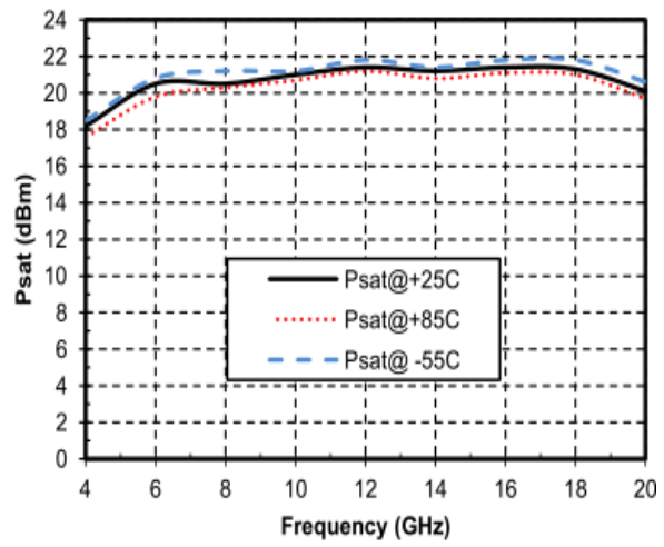
Psat vs. Frequency
