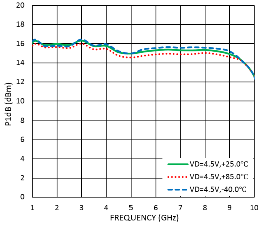
Measurement Plots: P1dB VD=4.5V
