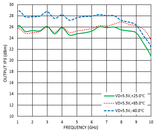
Measurement Plots: OIP3 VD=5.5V
