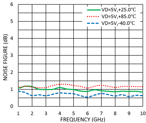
Measurement Plots: Noise Figure VD=5V
