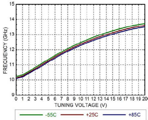
Frequency vs. Tuning Voltage VDD=+5V
