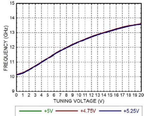
Frequency vs. Tuning Voltage T=25°C
