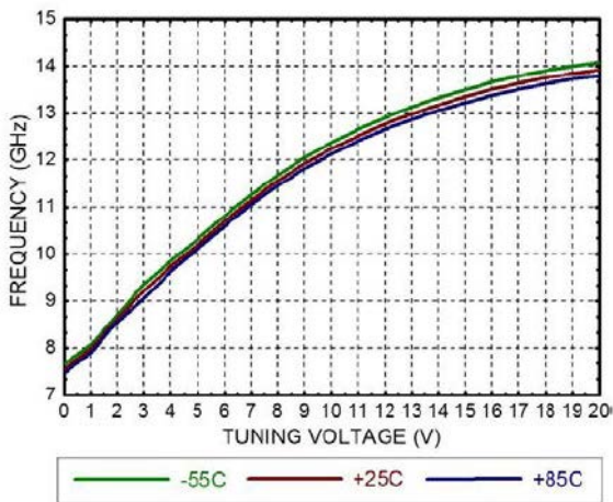
Output Frequency Curve at Mode1
