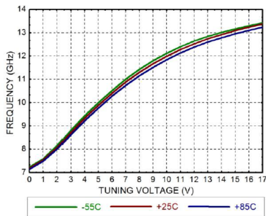
Output Frequency Curve at Mode2
